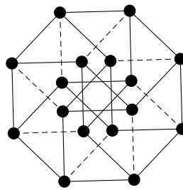
Figure 3.6: The sporadic maximal connected cyclotomic \mathbb{Z} -hypercube S_{16} .
