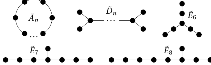
Figure 1.1: Extended simply-laced Coxeter graphs
